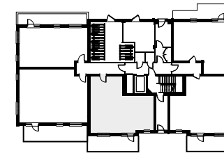
MILL HOUSE GROUND FLOOR – APARTMENT 1
