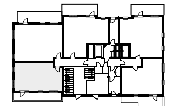
RIVIERA HOUSE GROUND FLOOR – APARTMENT 3
