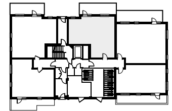
CRANEFORD HOUSE GROUND FLOOR – APARTMENT 1
